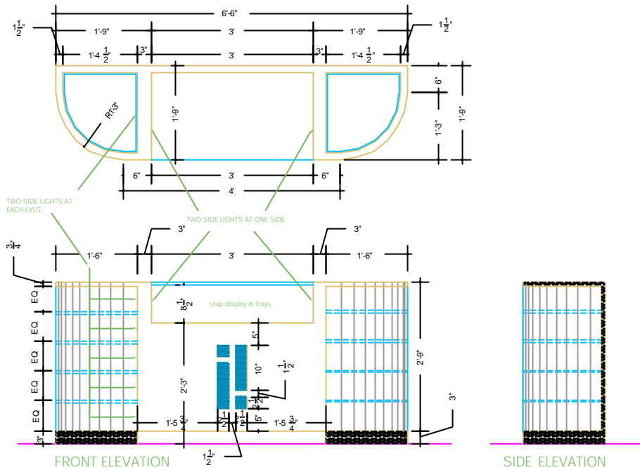
FRONT ELEVATION
